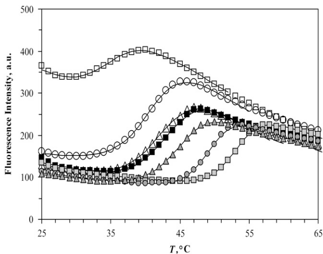
FIGURE 6 Temperature denaturation profiles of Plk1-PBD ( 10 \mu\text{M} ). Black-filled symbols represent the denaturation profile of Plk1-PBD without added ligand. Addition of the ligand ANS (open symbols) destabilized the protein, shifting the T_m downward, whereas the addition of the phosphorylated peptide (gray solid symbols) stabilized the protein, shifting its T_m upward. The concentrations of the ligands: (triangles) 15.6 \mu\text{M} peptide and 31.3 \mu\text{M} ANS, (circles) 100 \mu\text{M} , (squares) 1000 \mu\text{M} . Data points are experimental observations; the lines are simulated according to the model of Eq. 13. The denaturation parameters of free Plk1-PBD were T_m = 43.28^\circ\text{C} and \Delta_U H_{T_i} = 330 \text{ kJ/mol} .
