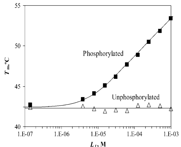
FIGURE 8 Dependence of the Plk1-PBD melting temperature on the concentration of added peptide in two forms: phosphorylated (■) and unphosphorylated (△). Lines are drawn according to the model of Eq. 13, using the following parameters: \Delta_U H_{T_i} = 330 \text{ kJ/mol} , \Delta_{bN} H_{T_0} = -42 \text{ kJ/mol} , T_i = 43^\circ\text{C} , \Delta_U C_{p-T_i} = 6.3 \text{ kJ/(mol} \times \text{K)} , and \Delta_{bN} C_{p-T_0} = -1.3 \text{ kJ/(mol} \times \text{K)} . For phosphorylated peptide, the binding constant was K_{bN} = 2.3 \times 10^5 \text{ M}^{-1} . The unphosphorylated peptide binding constant was nondetectable ( K_{bN} \ll 10^2 \text{ M}^{-1} ).
