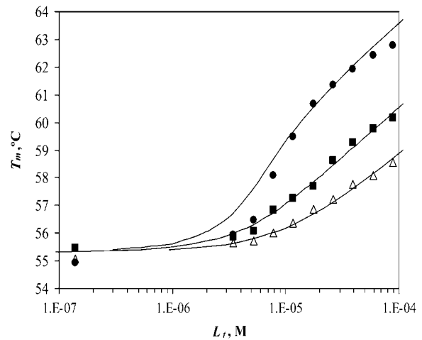
FIGURE 7 Dependence of the hCAII melting temperature on ligand concentration: AZM (●), 3d (■), and CARBS (△). Lines are drawn according to the model of Eq. 13. Regressed values of ligand binding constants ( K_{bN-T_0} ) are 6 \times 10^6 , 8 \times 10^5 , and 2.5 \times 10^5 for AZM, 3d, and CARBS, respectively.
